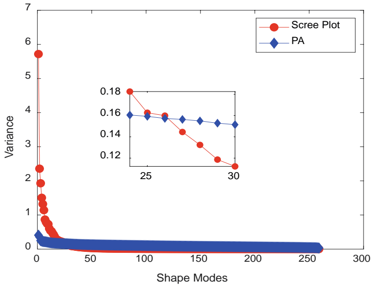
Figure 1. Parallel analysis
