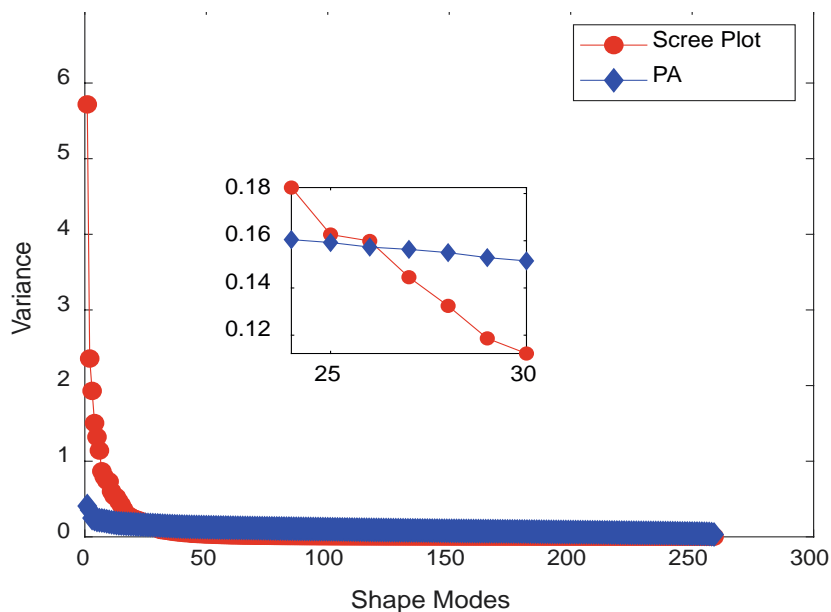
Figure 1. Parallel analysis.
